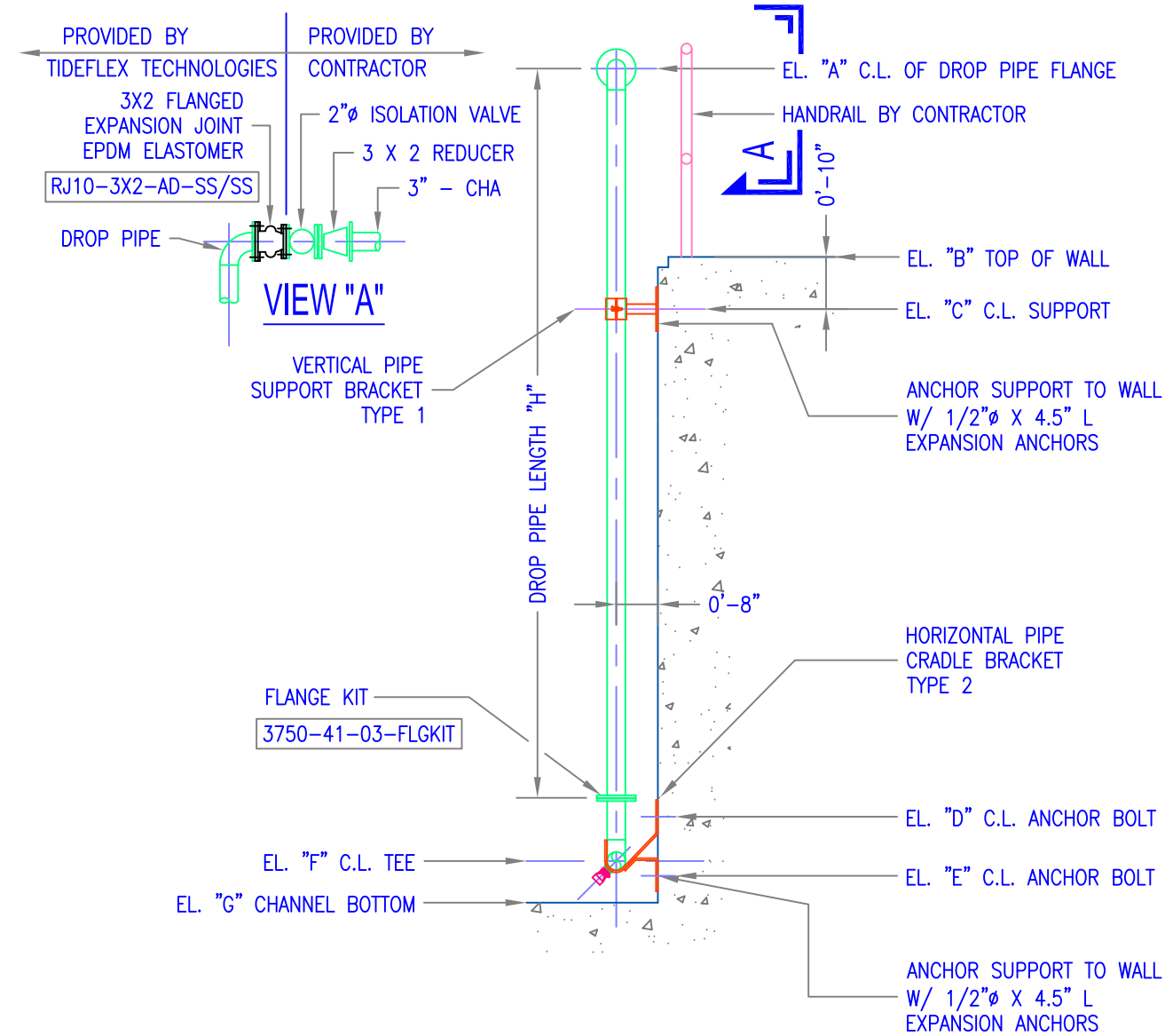
ELEVATION - MANIFOLD ASSEMBLY
