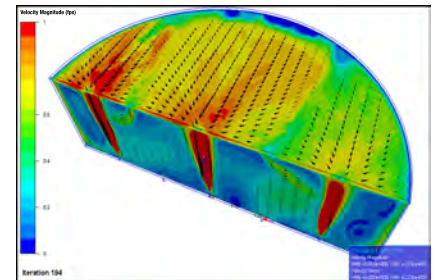
CFD Model
